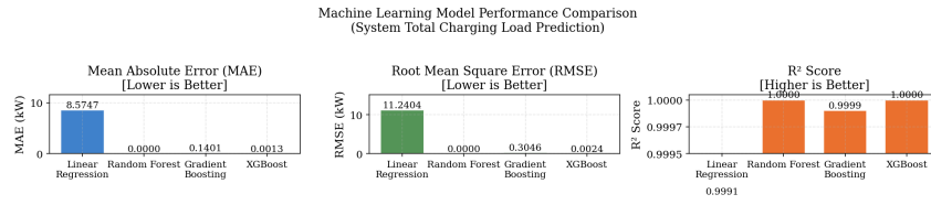
Figure 4.2: Comparison of ML model performance metrics (MAE, RMSE, R^2 ).
